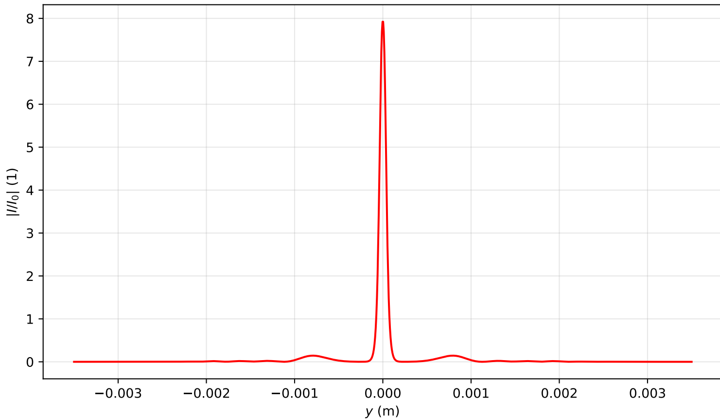
Intensity profile I(x=0, y, z=0.637)/I_0 , P_{in}=8.0P_{cr} , artificial time
